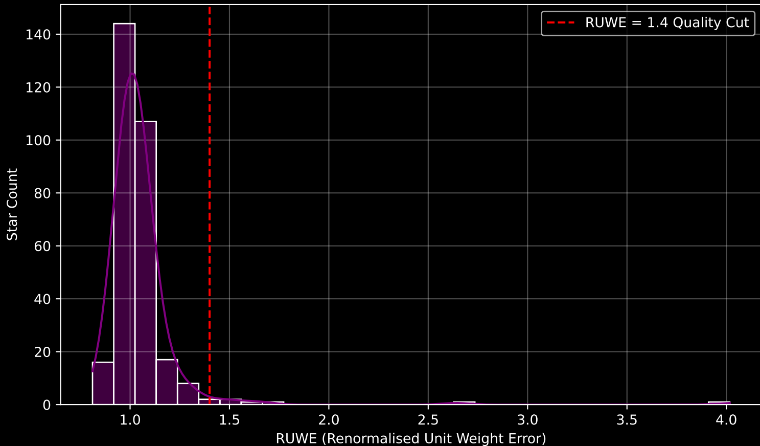
GAPOGEE DR17 Field [161+00] RUWE Distribution (n= 300)
