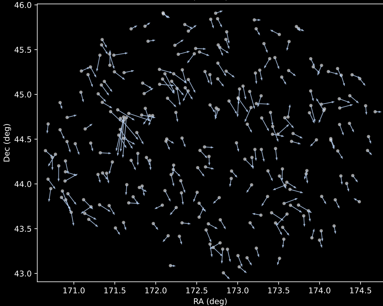
APOGEE DR17 Cluster 1 Proper Motion Vectors (n=256)
