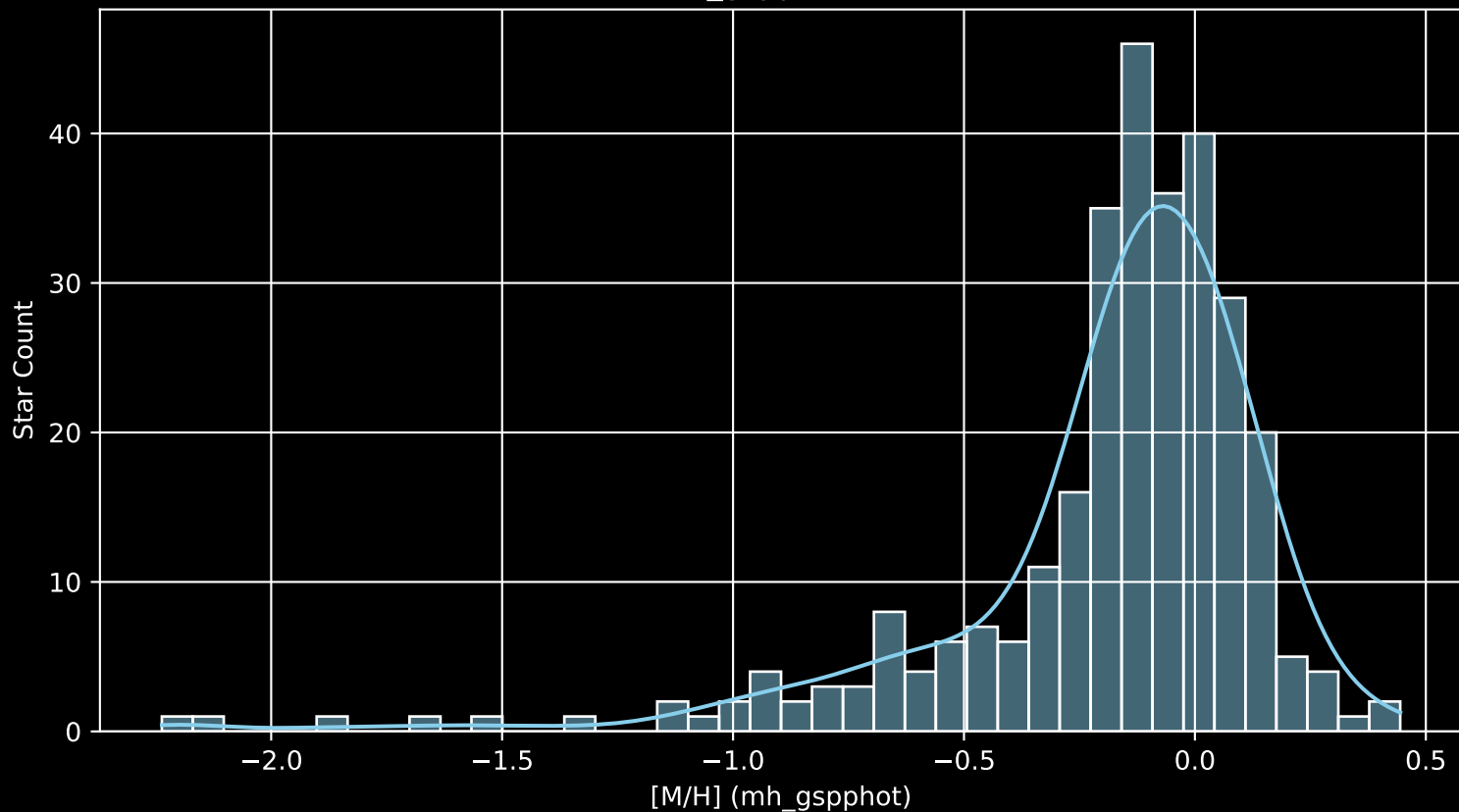
APOGEE DR17 Field: [161+00 [M/H] (mh_gspphot) (n= 299)
