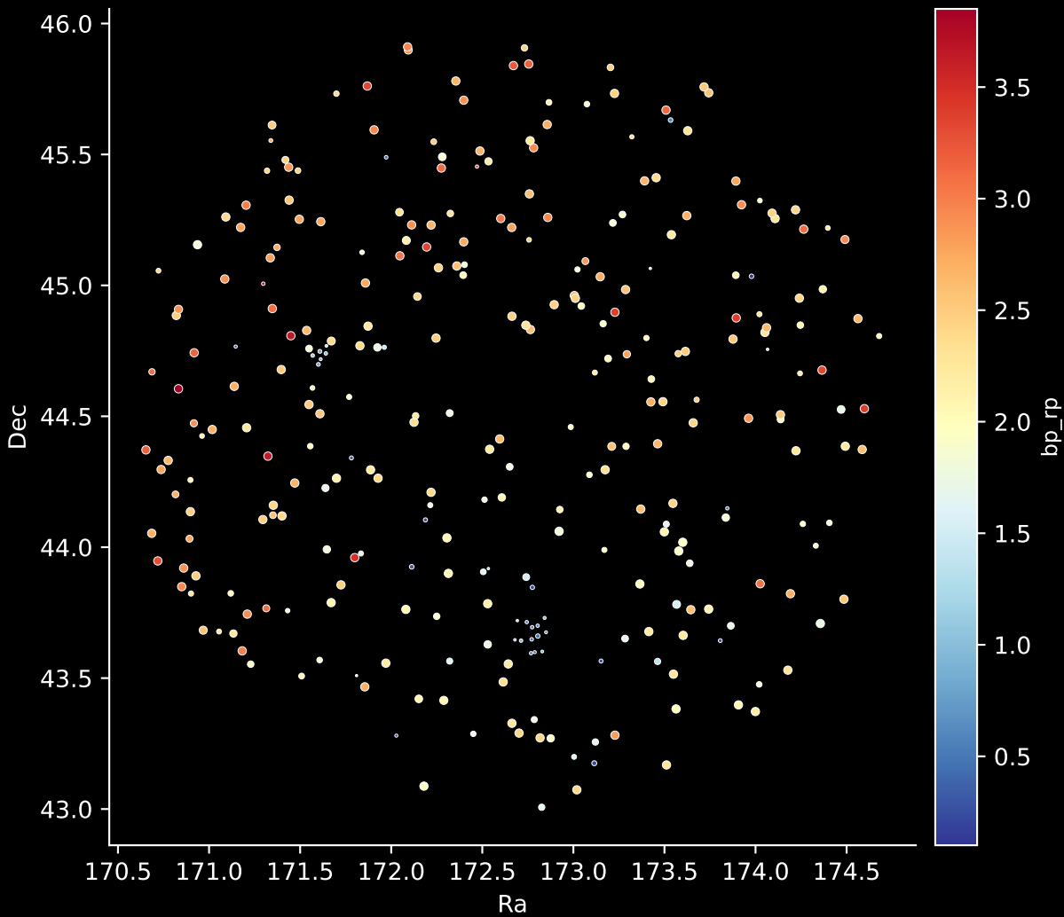
APOGEE DR17 Field: [161+00] Stars: 304
