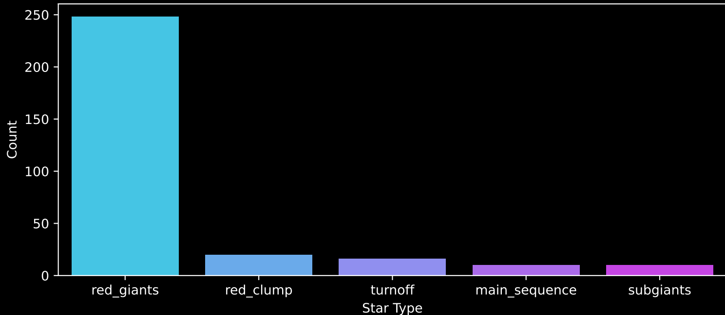
APOGEE DR17 Field: [161+00] Count plot of Star Type
