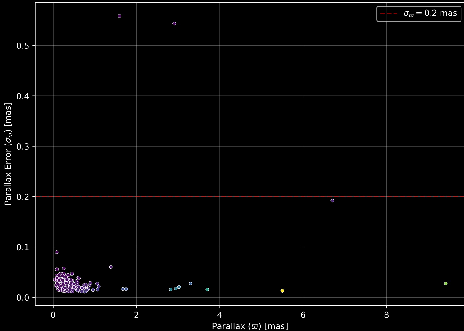
APOGEE DR17 Field: [161+00] Parallax Quality (n= 304)
