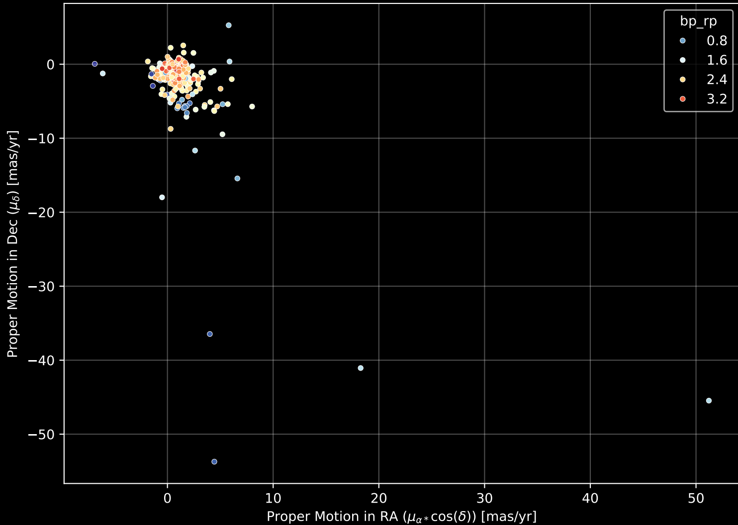
APOGEE DR17 Field: [161+00] Proper Motion Diagram (n= 304)
